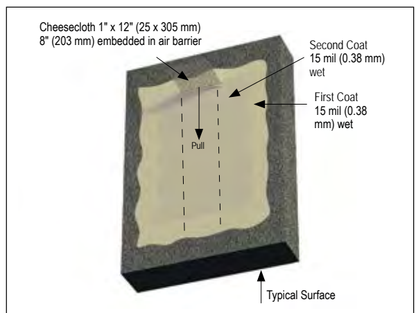
Figure 13. Adhesion Test Procedure Diagram
