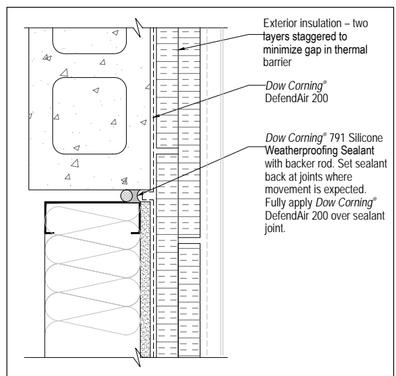
Figure 3. Change in Wall Substrate
