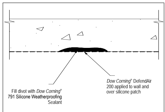
Figure 2. Divot in Concrete
