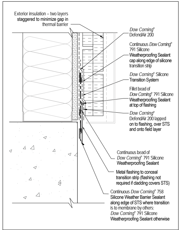
Figure 10. Stud Wall to Concrete Wall
