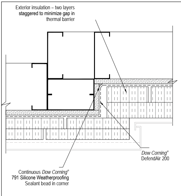
Figure 5. Vertical Wall Offset
