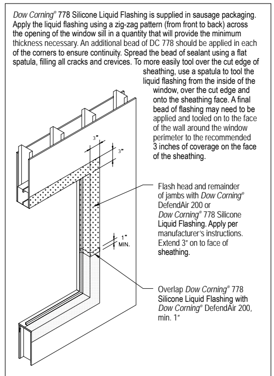
Figure 7. Window Opening – Isometric Sequencing Dow Corning® 778 Silicone Liquid Flashing
