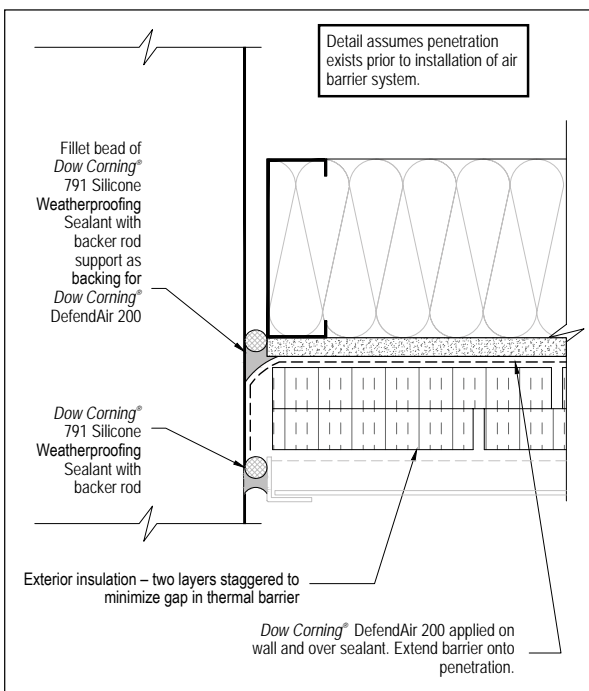
Figure 6. Vertical Wall Offset
