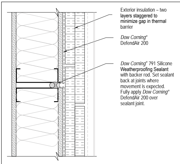
Figure 4. Control Joint
