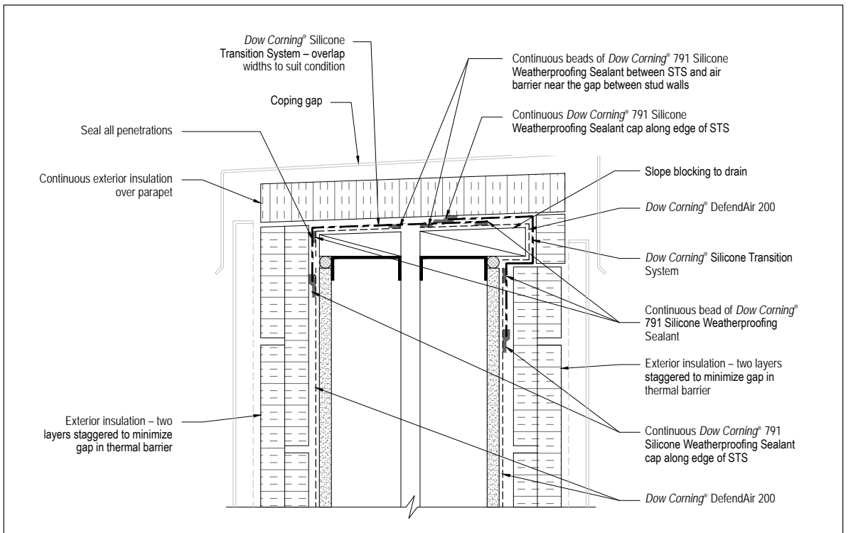
Figure 11. Dow Corning ® Silicone Transition System at Parapet
